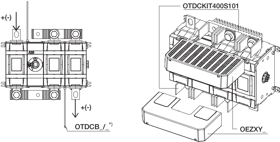
Circuit 5c, 5d Accessories for OTDC250...400U
