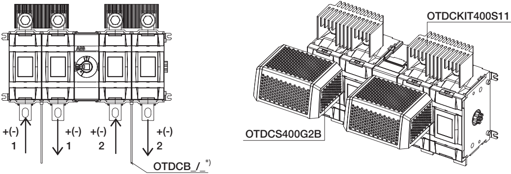
Circuit 3 Accessories for OTDC315...500E, OTDC250...400U
