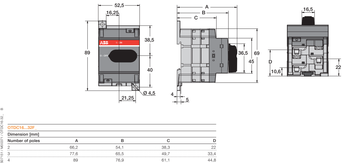
OTDC16...32F_, base or DIN-rail mounting (IEC)
