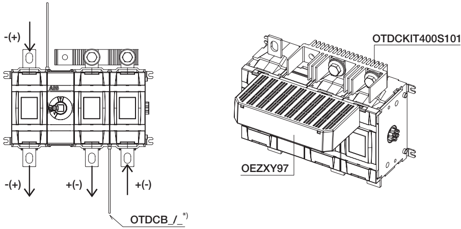
Circuit 5a, 5b, 5e Accessories for OTDC315...500E, OTDC250...400U
