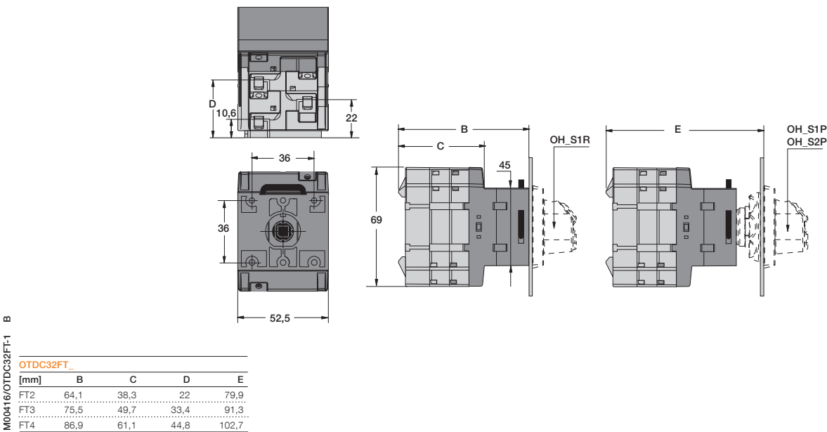
OTDC16...32FT_, door mounting (IEC)
