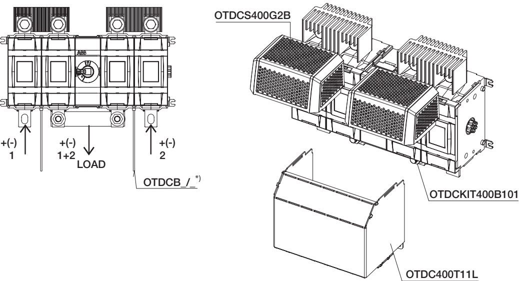
Circuit 6f Accessories for OTDC250...400US
